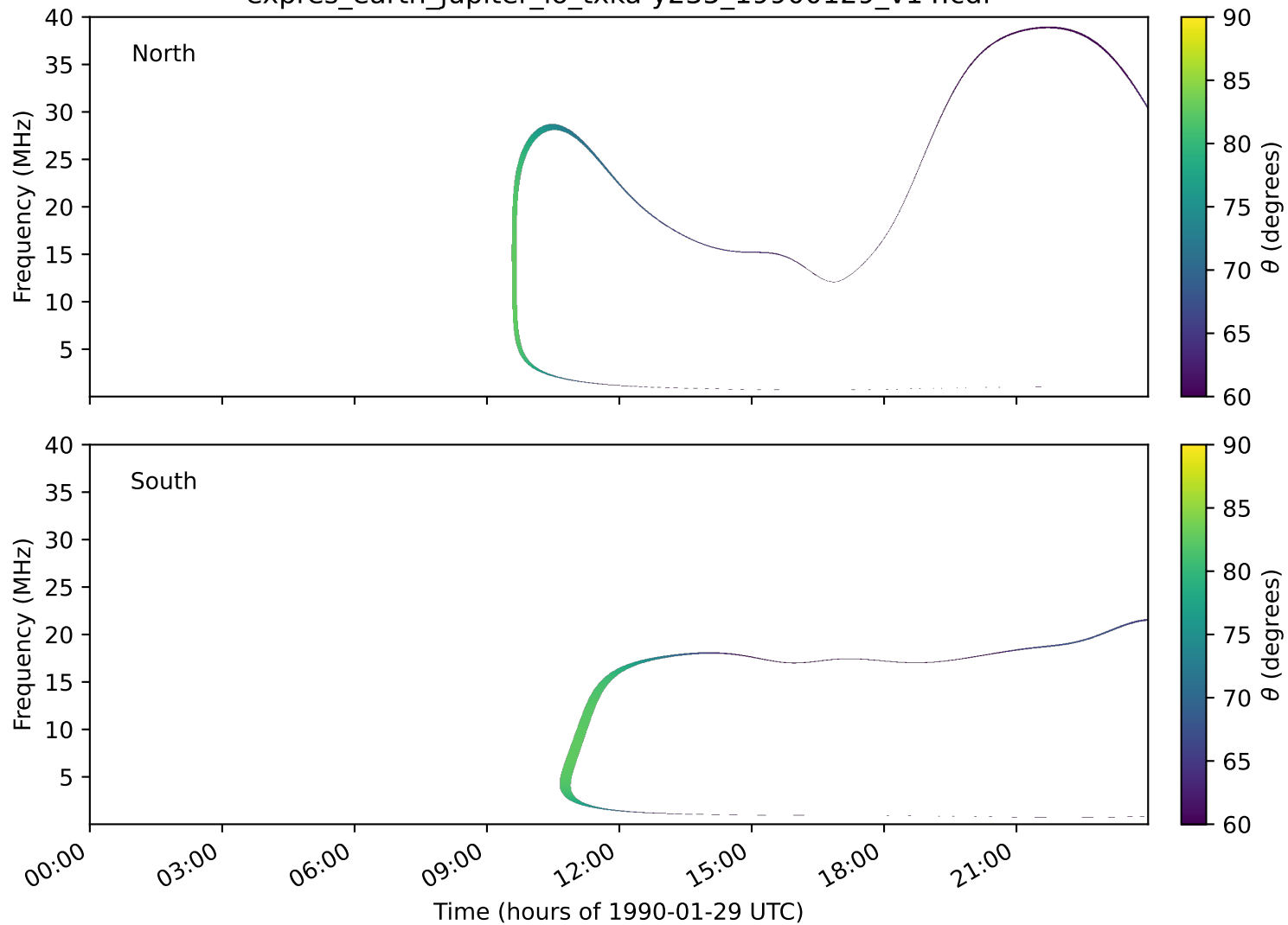
expres_earth_jupiter_io_txka-y235_19900129_v14.cdf
