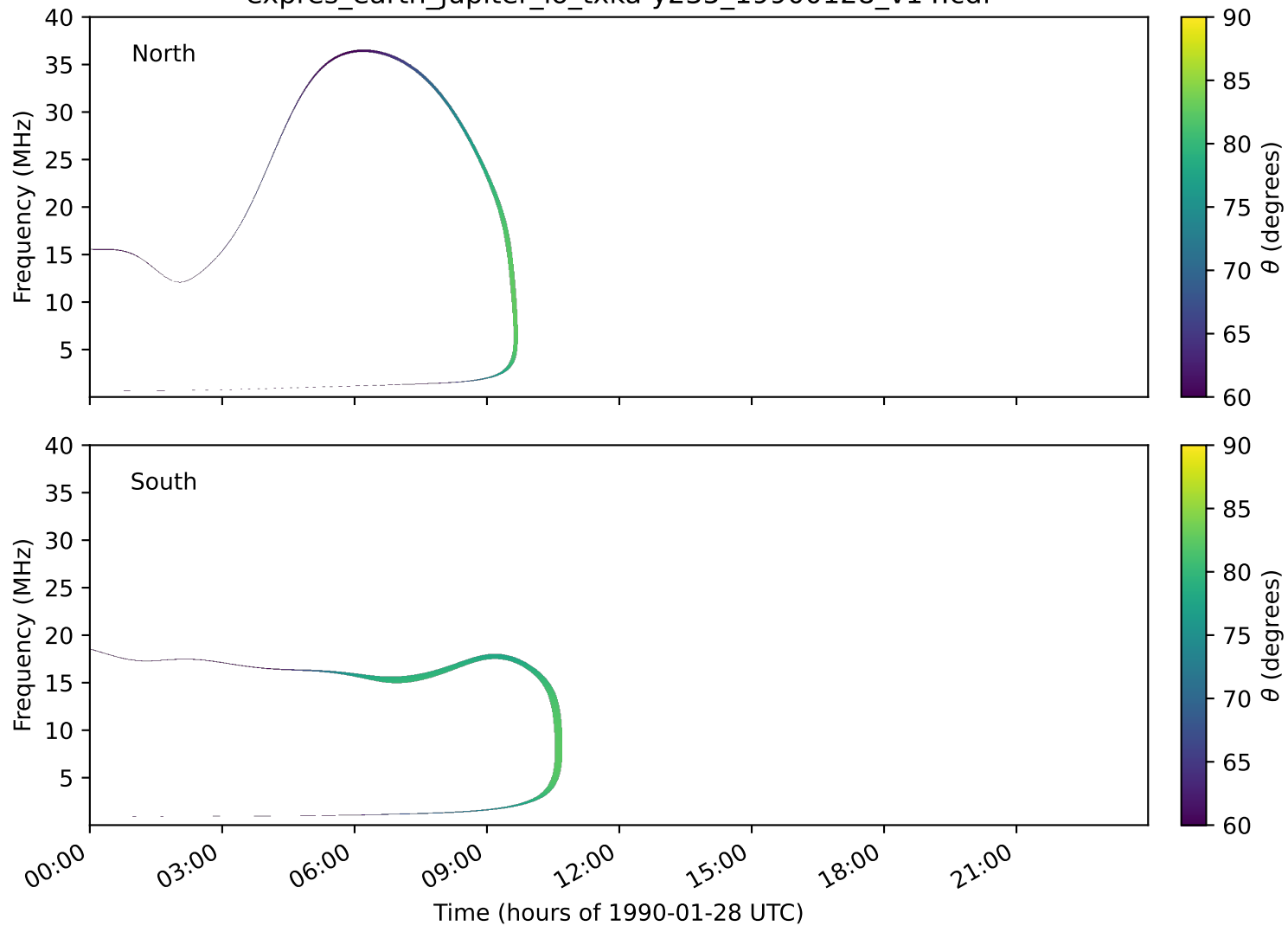
expres_earth_jupiter_io_txka-y235_19900128_v14.cdf
