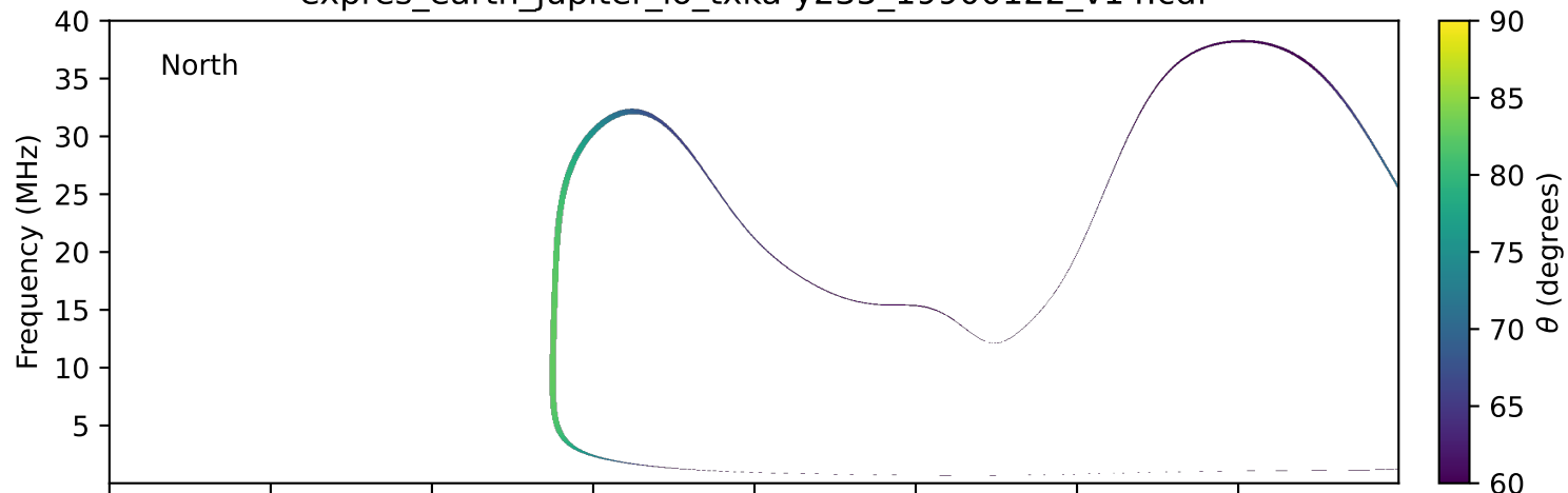
expres_earth_jupiter_io_txka-y235_19900122_v14.cdf
