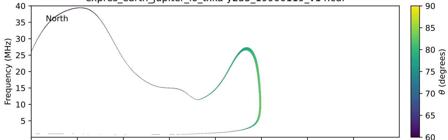
expres_earth_jupiter_io_txka-y235_19900119_v14.cdf
