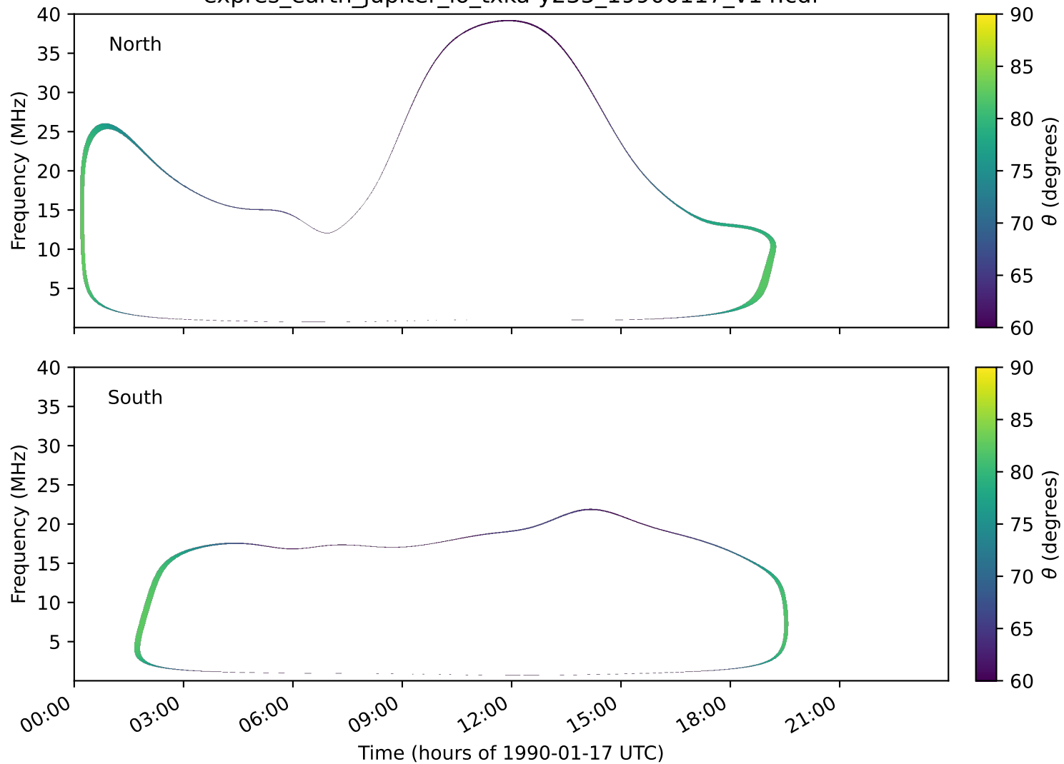
expres_earth_jupiter_io_txka-y235_19900117_v14.cdf
