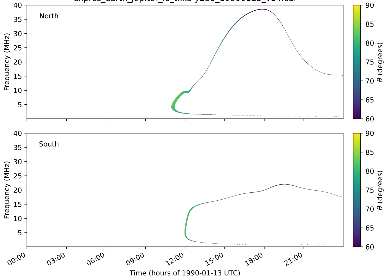
expres_earth_jupiter_io_txka-y235_19900113_v14.cdf
