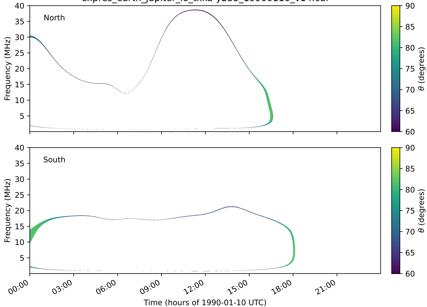
expres_earth_jupiter_io_txka-y235_19900110_v14.cdf
