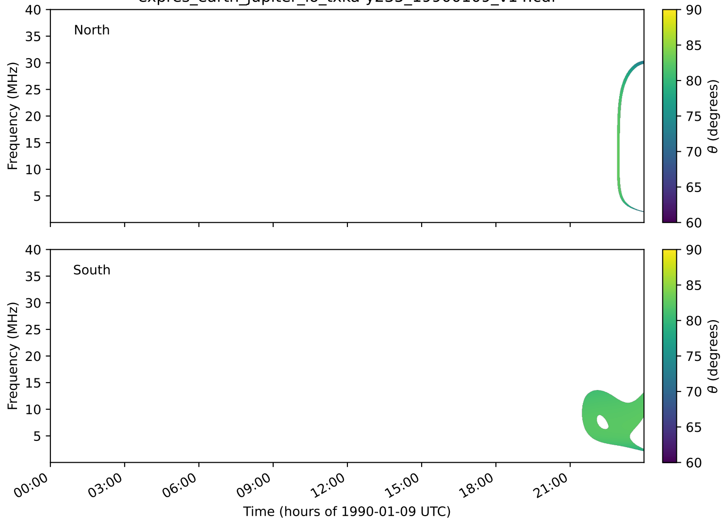
expres_earth_jupiter_io_txka-y235_19900109_v14.cdf
