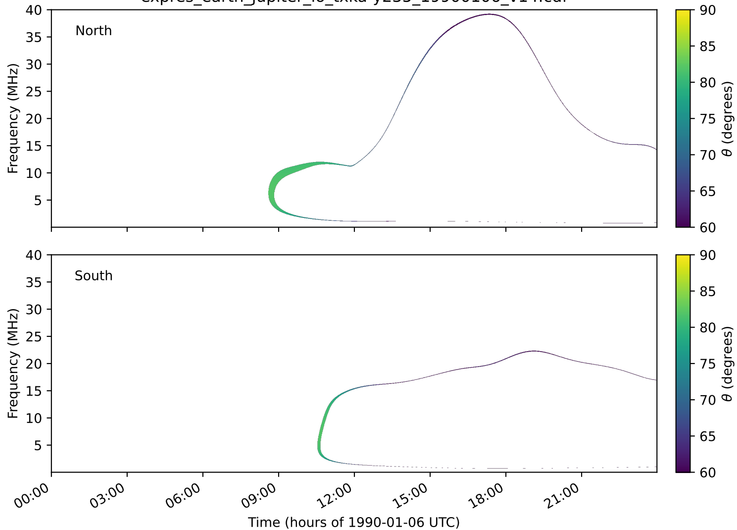
expres_earth_jupiter_io_txka-y235_19900106_v14.cdf
