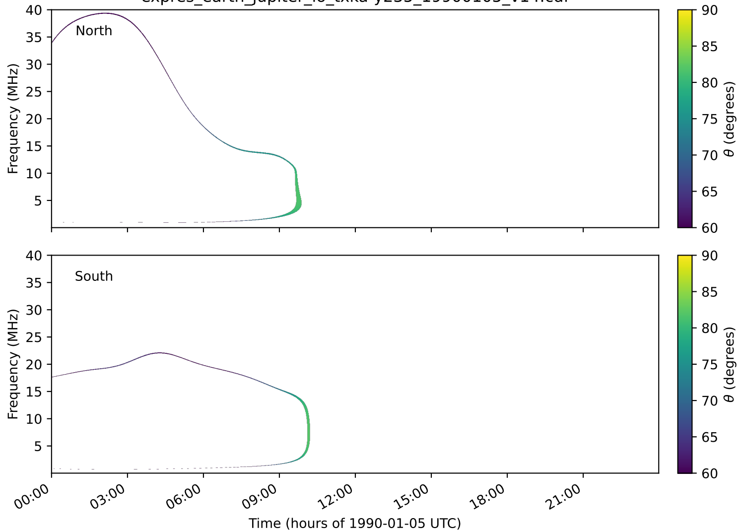
expres_earth_jupiter_io_txka-y235_19900105_v14.cdf
