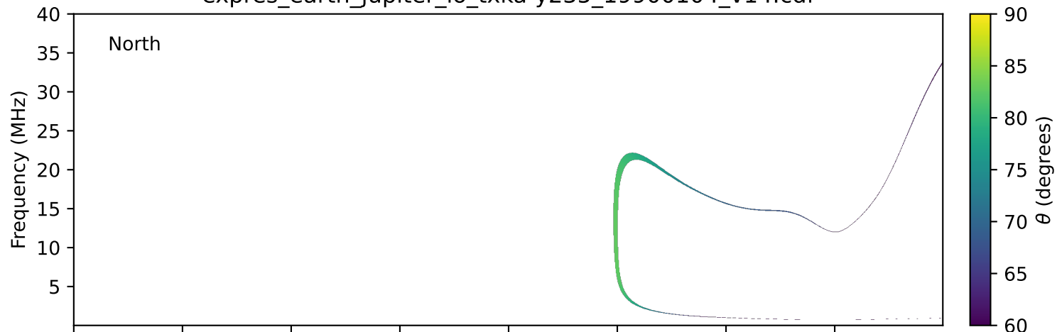
expres_earth_jupiter_io_txka-y235_19900104_v14.cdf
