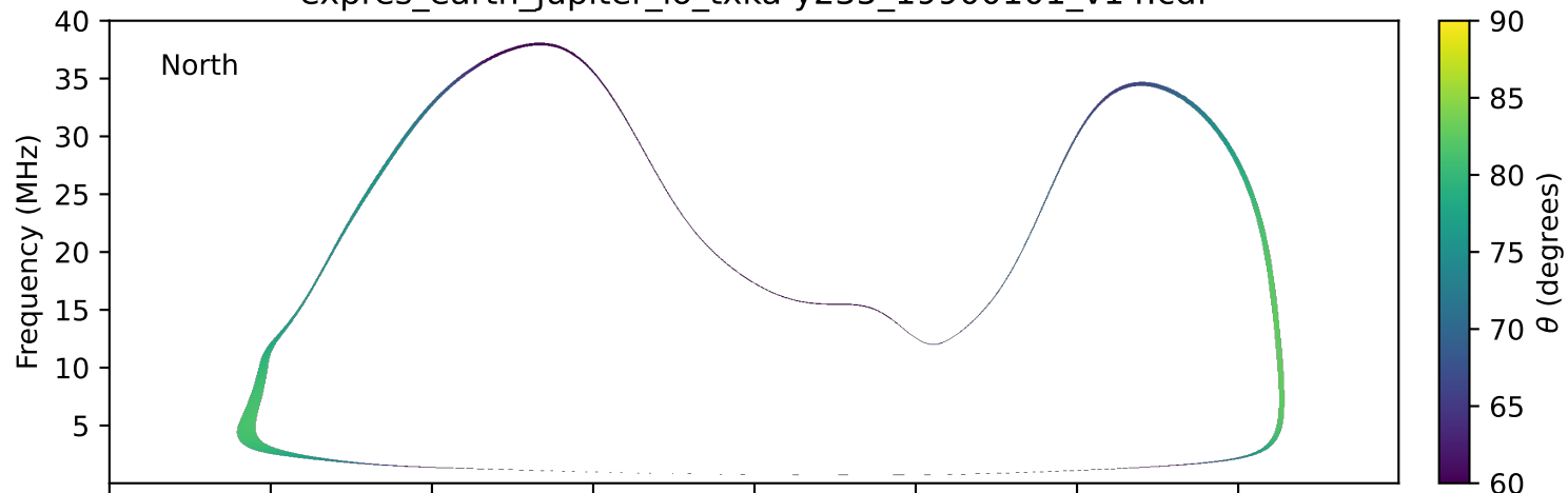
expres_earth_jupiter_io_txka-y235_19900101_v14.cdf
