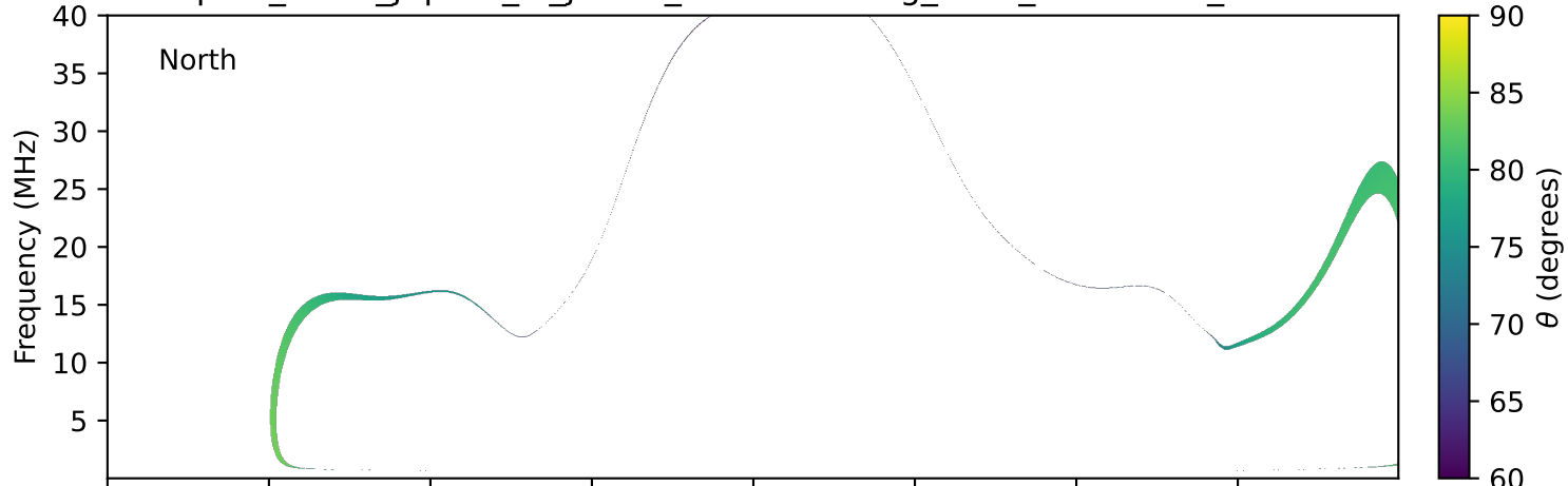
expres_earth_jupiter_io_jrm33_lossc-wid1deg_3kev_19900131_v11.cdf
