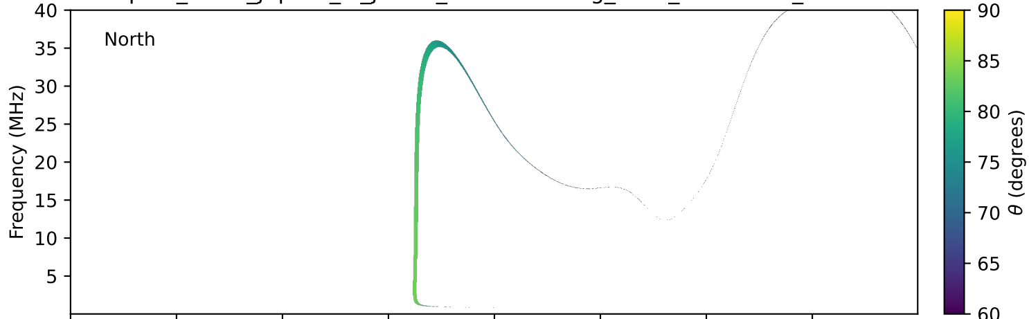
expres_earth_jupiter_io_jrm33_lossc-wid1deg_3kev_19900129_v11.cdf
