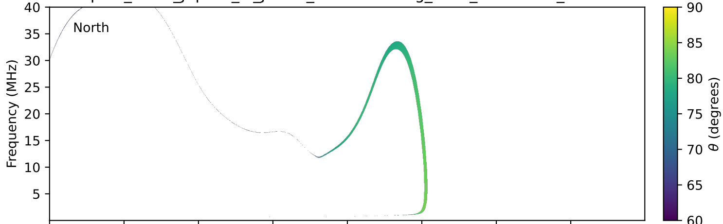
expres_earth_jupiter_io_jrm33_lossc-wid1deg_3kev_19900119_v11.cdf
