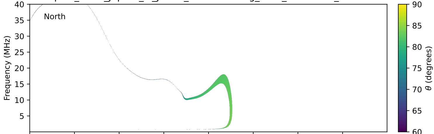
expres_earth_jupiter_io_jrm33_lossc-wid1deg_3kev_19900112_v11.cdf
