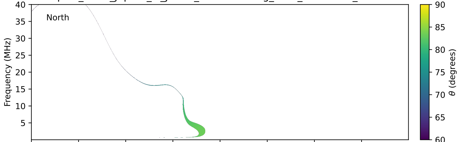
expres_earth_jupiter_io_jrm33_lossc-wid1deg_3kev_19900105_v11.cdf
