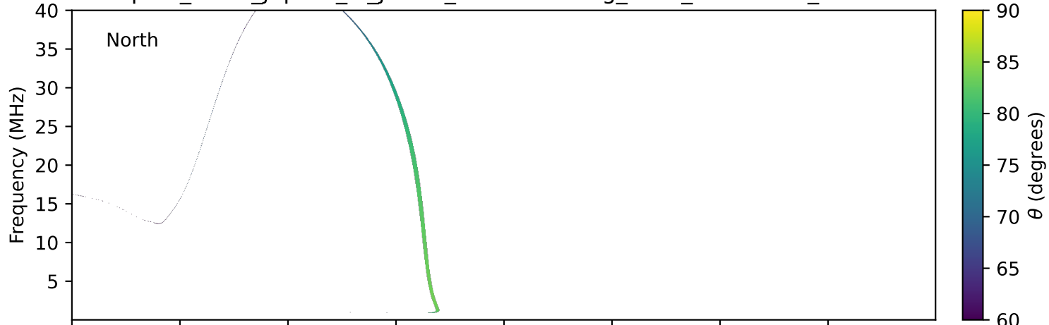
expres_earth_jupiter_io_jrm09_lossc-wid1deg_3kev_19900128_v11.cdf
