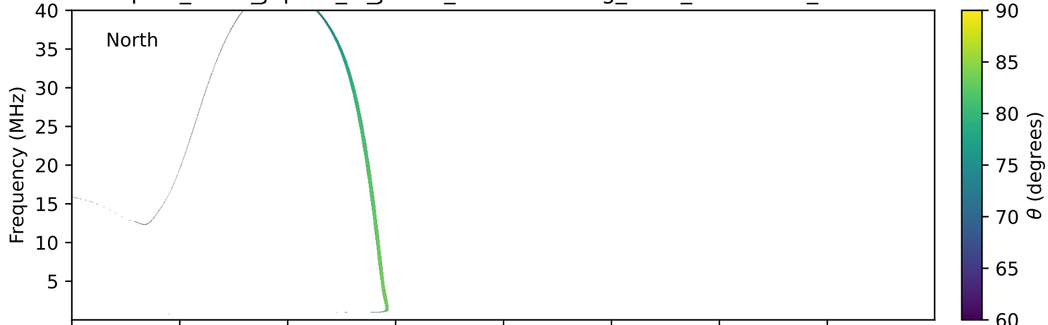
expres_earth_jupiter_io_jrm09_lossc-wid1deg_3kev_19900121_v11.cdf
