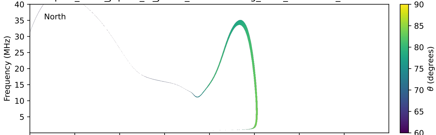
expres_earth_jupiter_io_jrm09_lossc-wid1deg_3kev_19900119_v11.cdf
