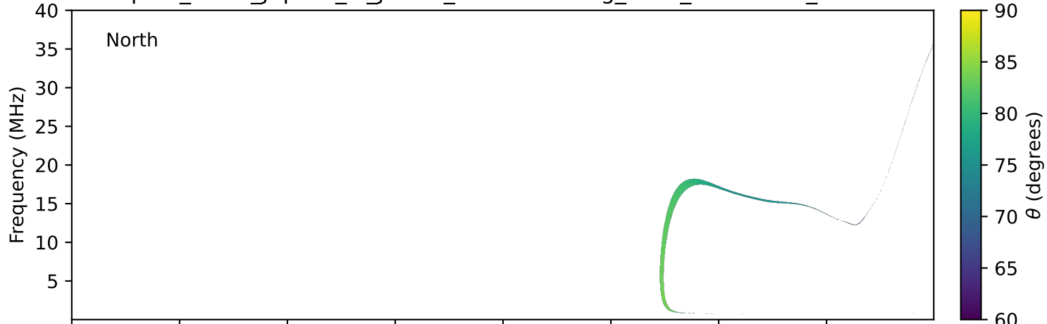
expres_earth_jupiter_io_jrm09_lossc-wid1deg_3kev_19900111_v11.cdf
