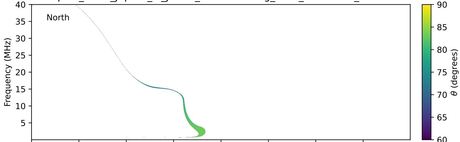
expres_earth_jupiter_io_jrm09_lossc-wid1deg_3kev_19900105_v11.cdf
