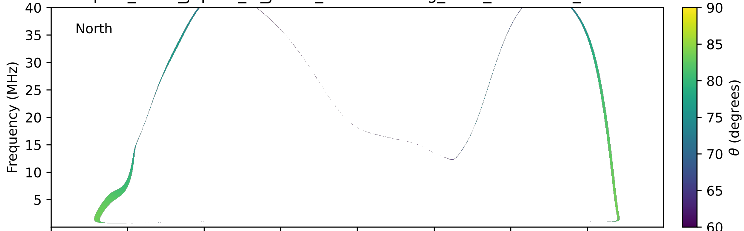
expres_earth_jupiter_io_jrm09_lossc-wid1deg_3kev_19900101_v11.cdf
