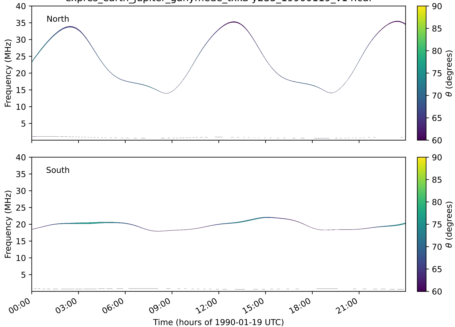
expres_earth_jupiter_ganymede_txka-y235_19900119_v14.cdf
