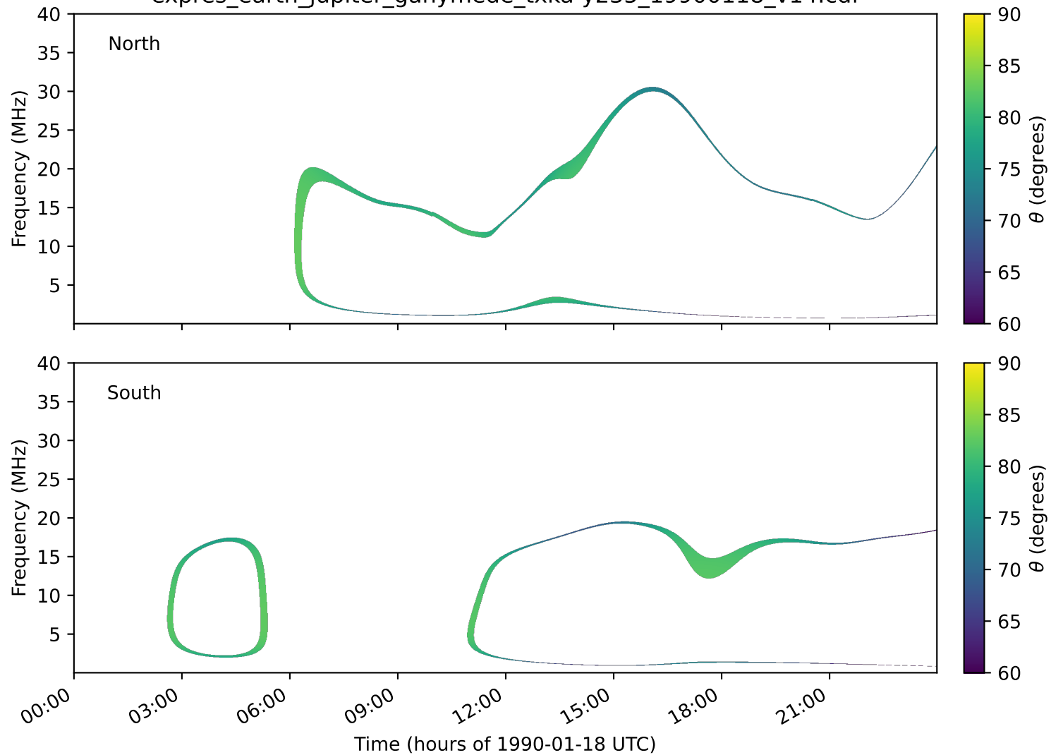
expres_earth_jupiter_ganymede_txka-y235_19900118_v14.cdf
