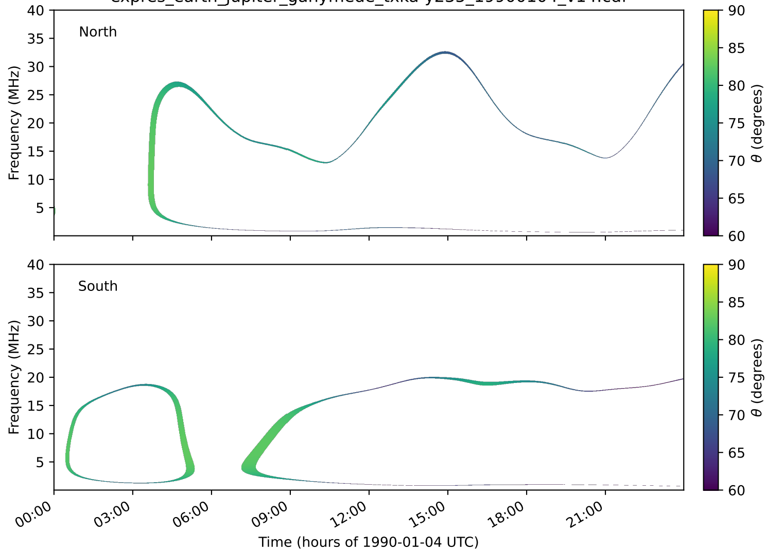
expres_earth_jupiter_ganymede_txka-y235_19900104_v14.cdf
