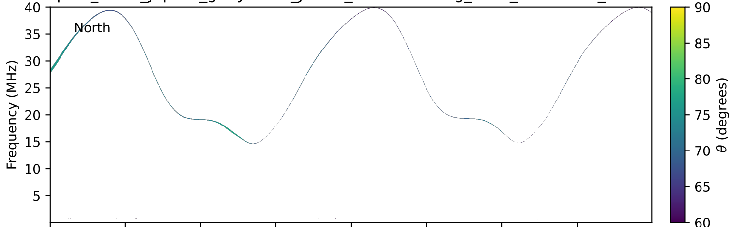
expres_earth_jupiter_ganymede_jrm33_lossc-wid1deg_3kev_19900119_v11.cdf
