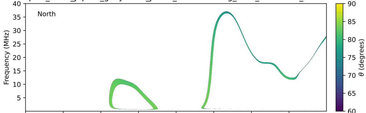
expres_earth_jupiter_ganymede_jrm33_lossc-wid1deg_3kev_19900118_v11.cdf
