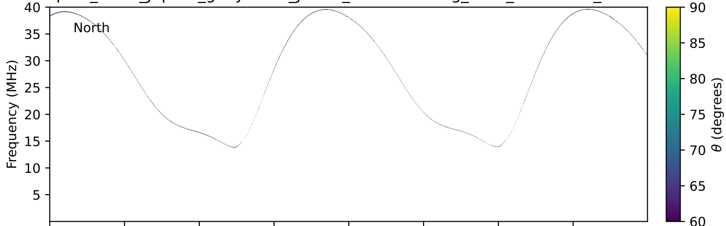
expres_earth_jupiter_ganymede_jrm09_lossc-wid1deg_3kev_19900105_v11.cdf
