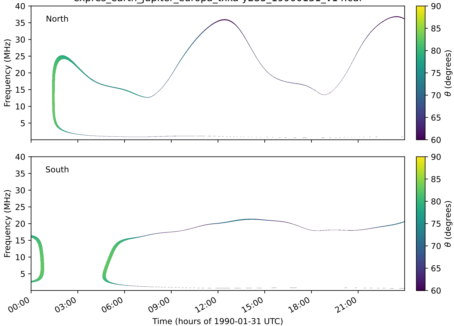
expres_earth_jupiter_europa_txka-y235_19900131_v14.cdf
