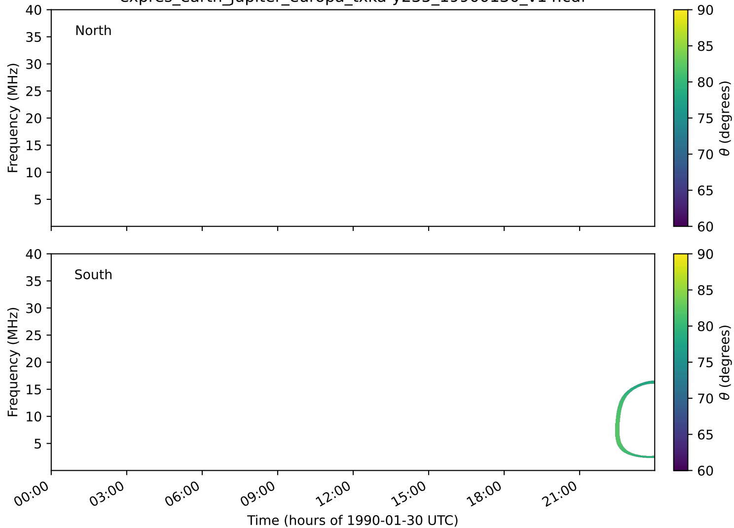
expres_earth_jupiter_europa_txka-y235_19900130_v14.cdf
