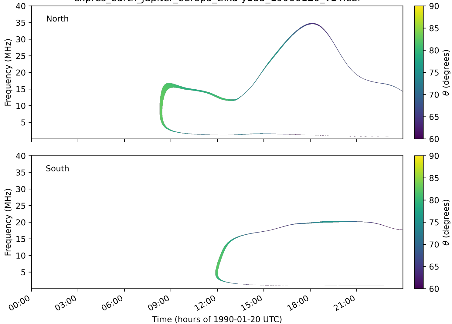
expres_earth_jupiter_europa_txka-y235_19900120_v14.cdf
