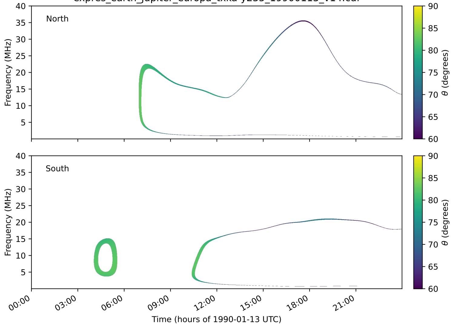
expres_earth_jupiter_europa_txka-y235_19900113_v14.cdf
