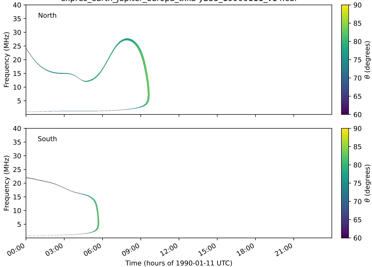
expres_earth_jupiter_europa_txka-y235_19900111_v14.cdf
