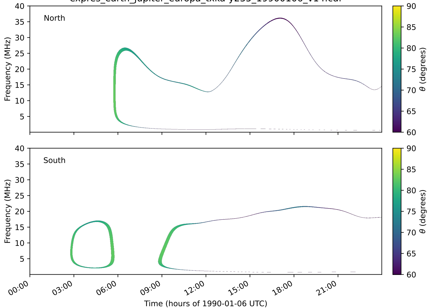
expres_earth_jupiter_europa_txka-y235_19900106_v14.cdf
