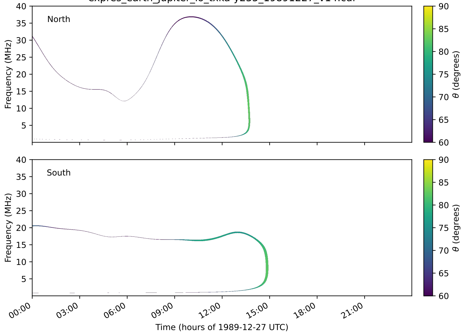
expres_earth_jupiter_io_txka-y235_19891227_v14.cdf
