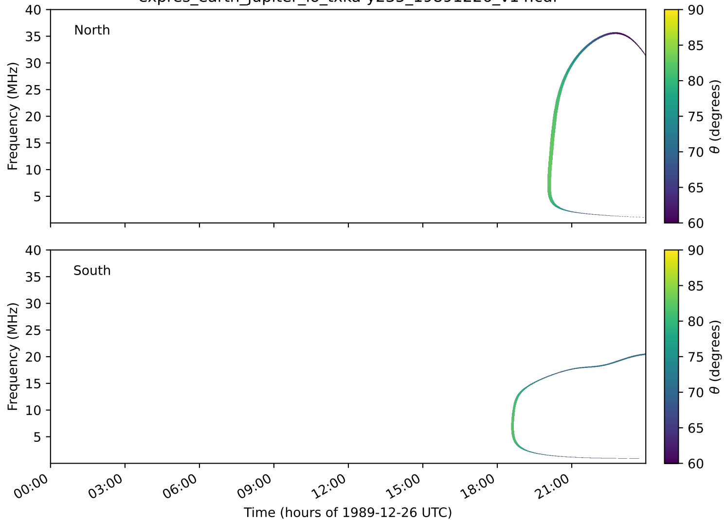
expres_earth_jupiter_io_txka-y235_19891226_v14.cdf
