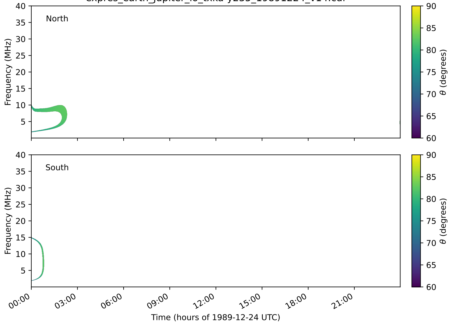
expres_earth_jupiter_io_txka-y235_19891224_v14.cdf
