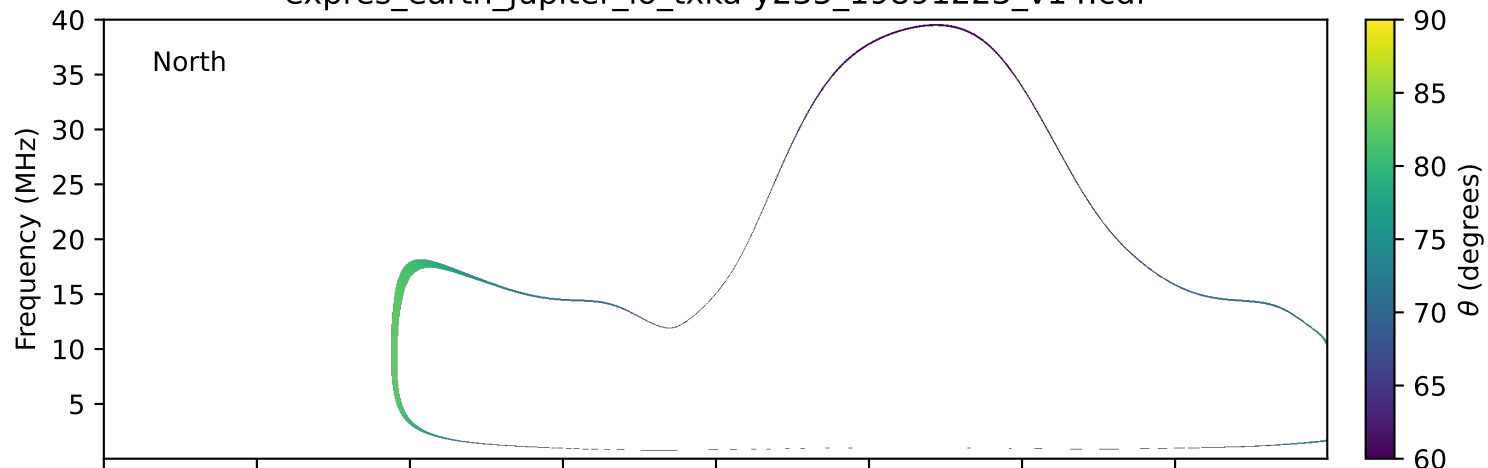
expres_earth_jupiter_io_txka-y235_19891223_v14.cdf
