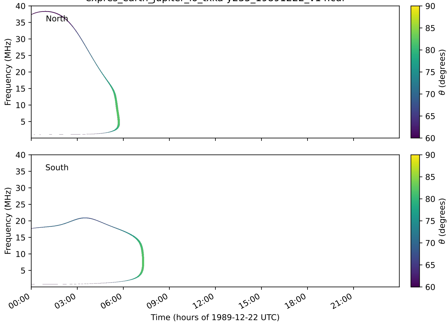
expres_earth_jupiter_io_txka-y235_19891222_v14.cdf
