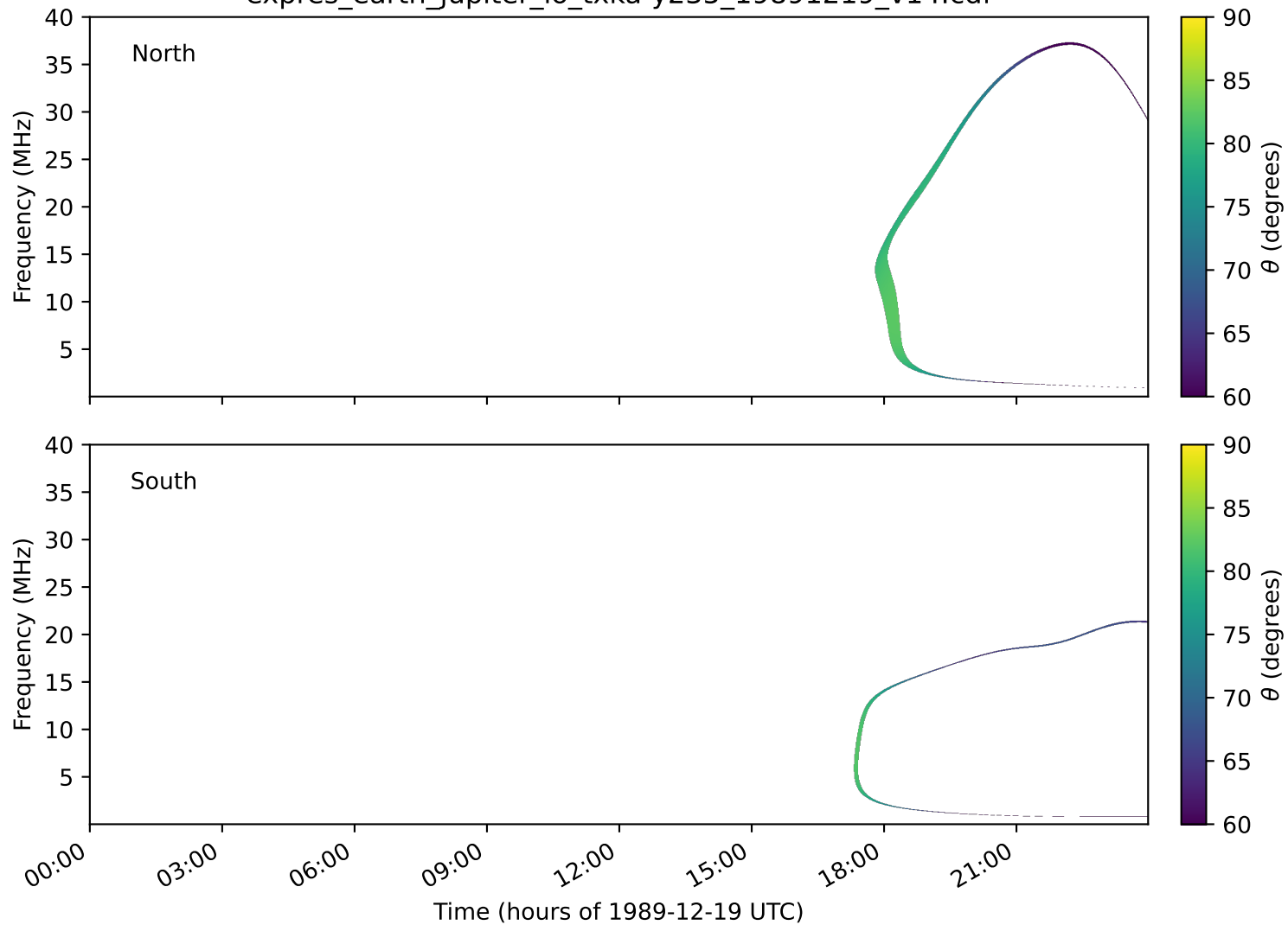
expres_earth_jupiter_io_txka-y235_19891219_v14.cdf
