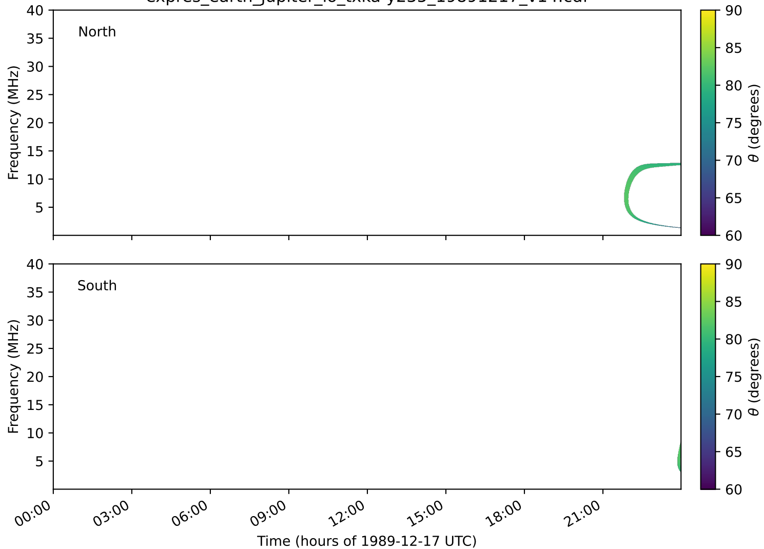
expres_earth_jupiter_io_txka-y235_19891217_v14.cdf
