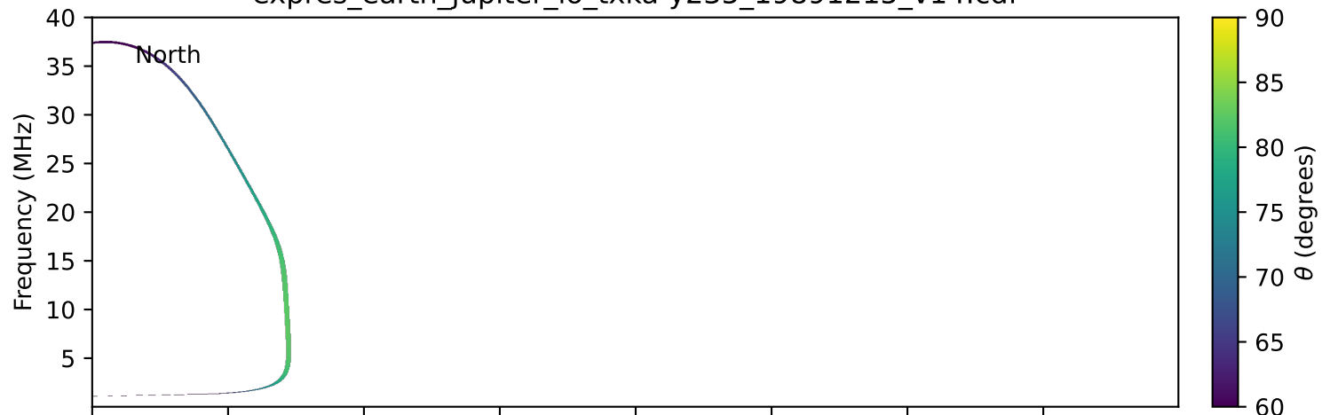
expres_earth_jupiter_io_txka-y235_19891215_v14.cdf
