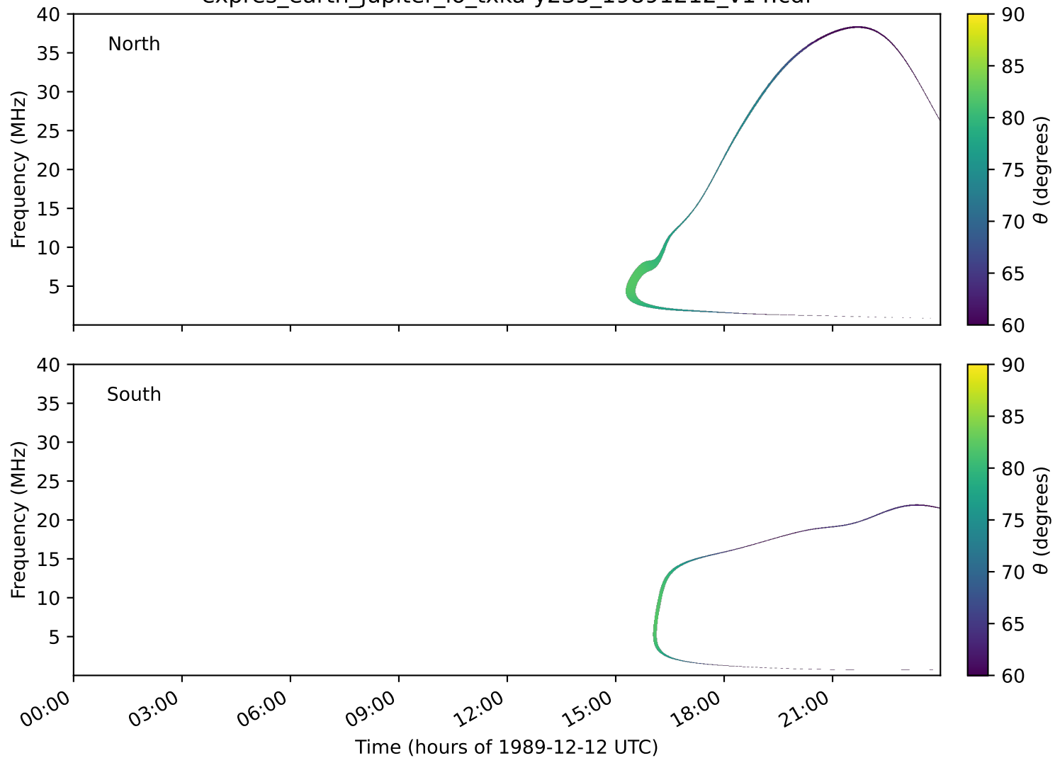
expres_earth_jupiter_io_txka-y235_19891212_v14.cdf
