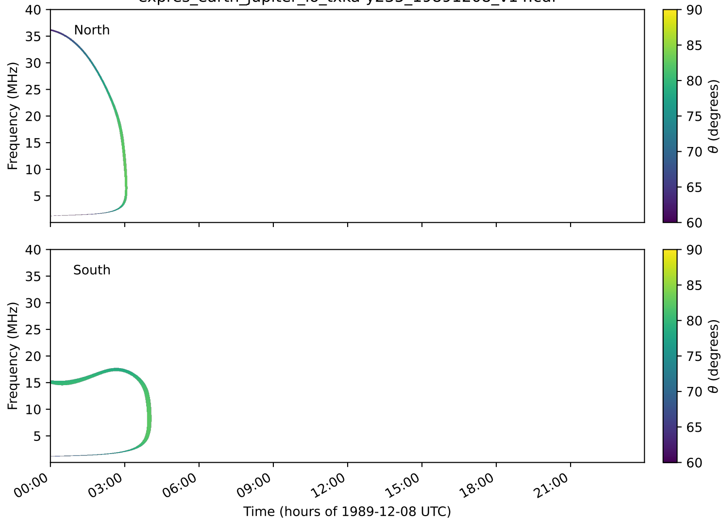
expres_earth_jupiter_io_txka-y235_19891208_v14.cdf
