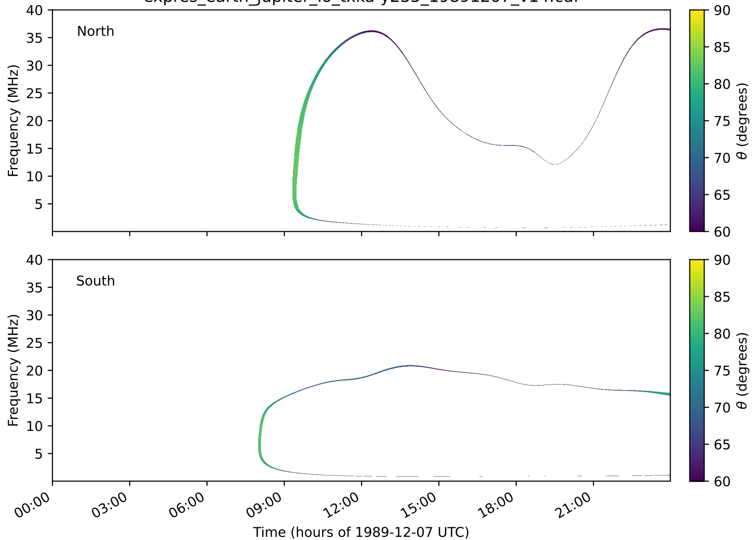
expres_earth_jupiter_io_txka-y235_19891207_v14.cdf
