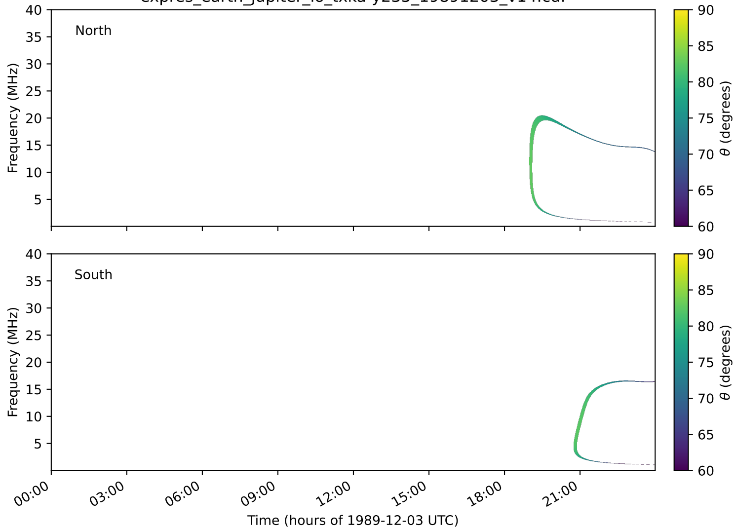
expres_earth_jupiter_io_txka-y235_19891203_v14.cdf
