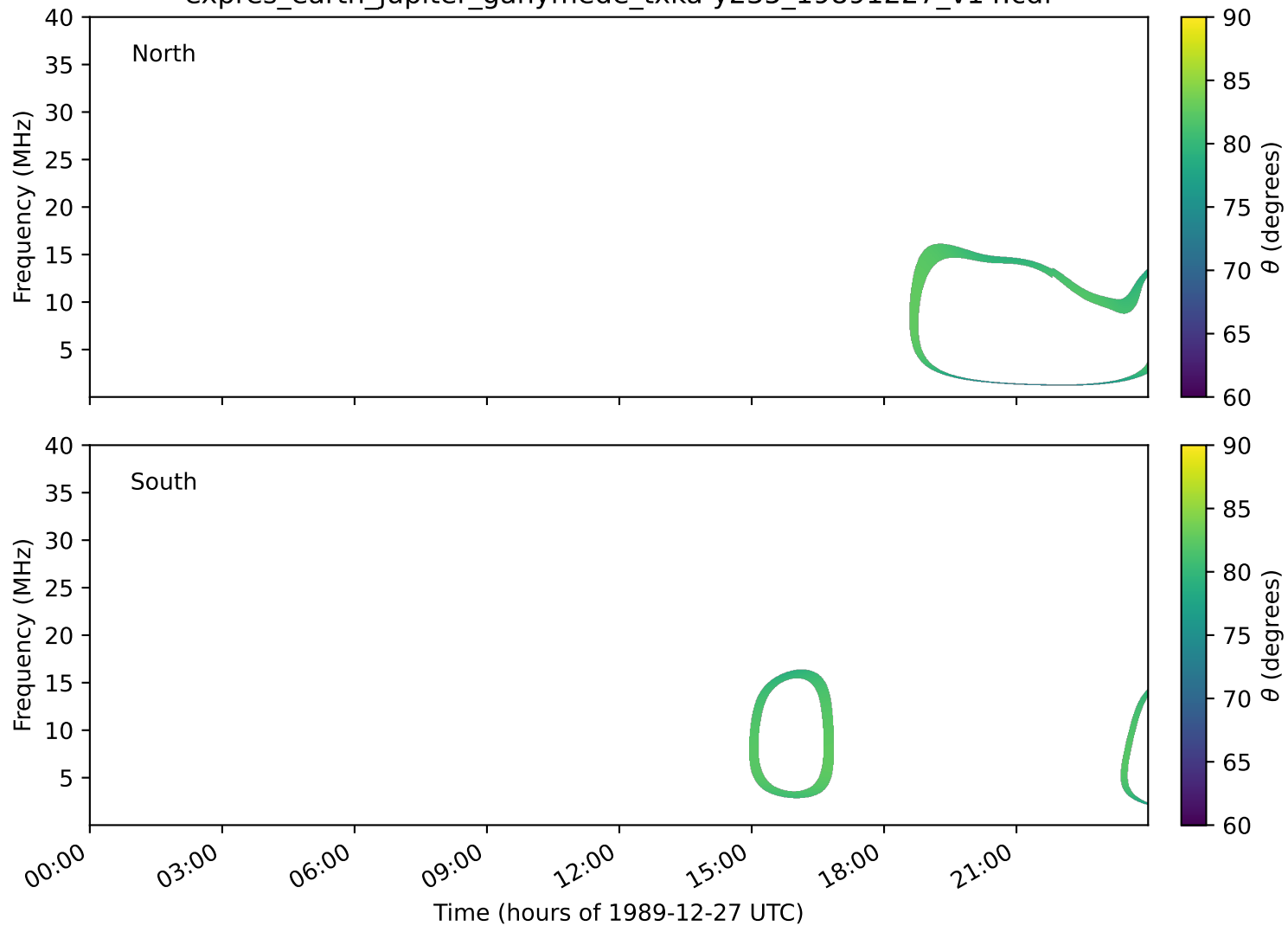
expres_earth_jupiter_ganymede_txka-y235_19891227_v14.cdf
