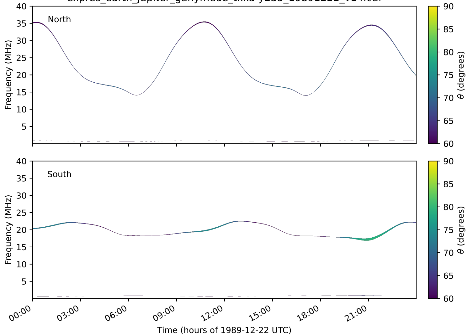
expres_earth_jupiter_ganymede_txka-y235_19891222_v14.cdf
