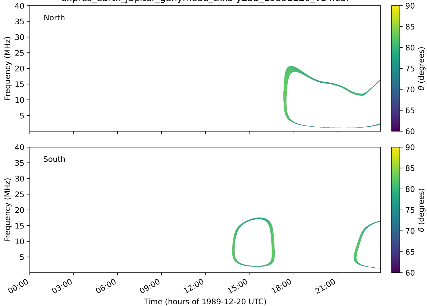
expres_earth_jupiter_ganymede_txka-y235_19891220_v14.cdf
